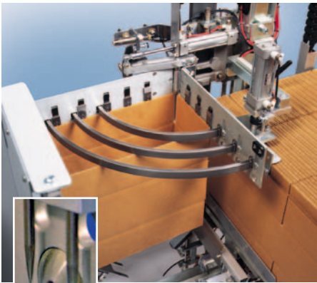
Our "Pin and Dome" technology, which provides a simple maintenance-free mechanical system, surpasses all other forms of case opening technologies.
